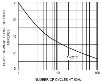
FIG.4-MAXIMUM FORWARD SURGE CURRENT
